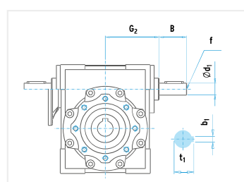
CRV-E/CMRV-E | Vite bisorgente / Double-end shaft
